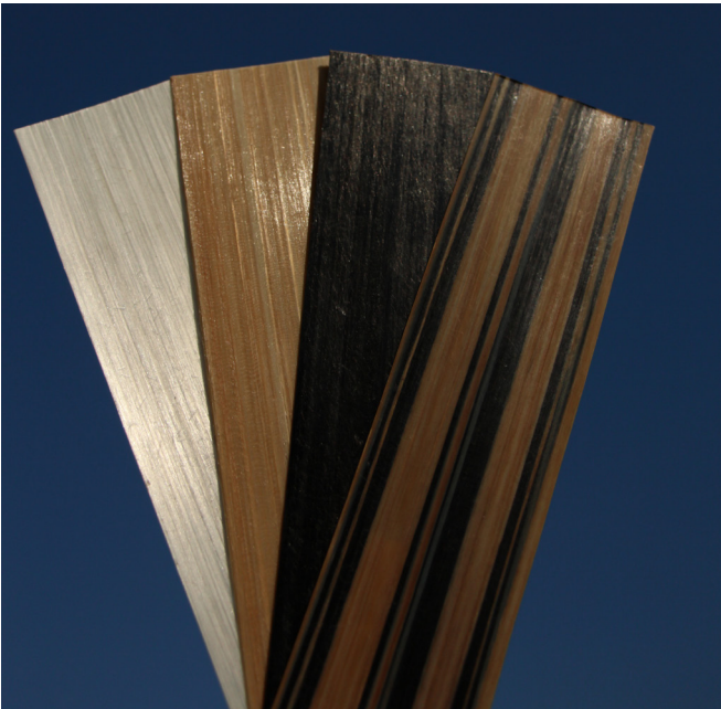
Thermoplastic tapes with different fiber matrix combinations. © Fraunhofer ICT | Picture in color and printing quality: www.fraunhofer.de/en/press
