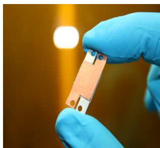
Micro battery with metal foil laminated housing © Fraunhofer IZM | Picture in color and printing quality: www.fraunhofer.de/en/press
