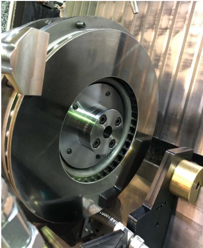
Picture 2: A finished brake disc coated with the EHLA process.
