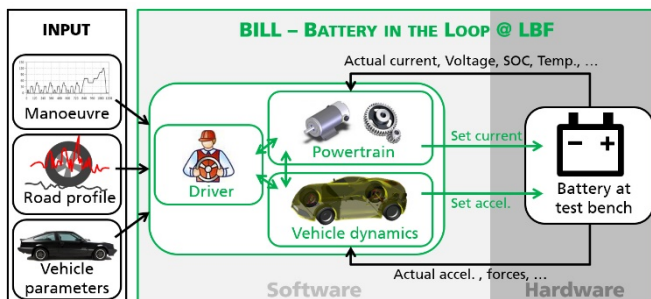
Picture 2: How the HiL-based (hardware-in-the-loop) test environment for traction batteries works.
