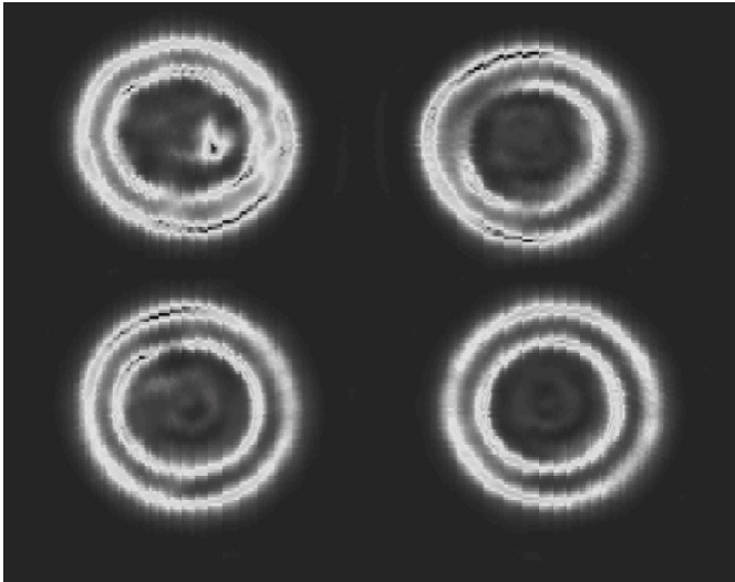
Picture 2: This radar image shows a glass splinter that was previously placed in the chocolate filling.
