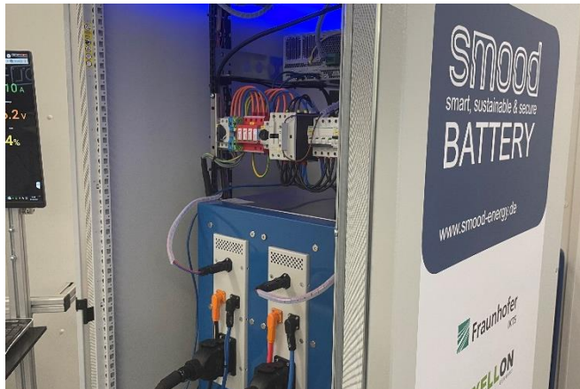
Fig. 2 The sodium-nickel chloride battery developed together with Fraunhofer IKTS in the EStorage joint research project will provide a sustainable, safe and inexpensive solution for energy storage.
