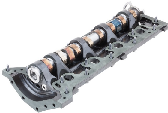
Picture 1: The camshaft module features a monolithic design with integrated bearings.
