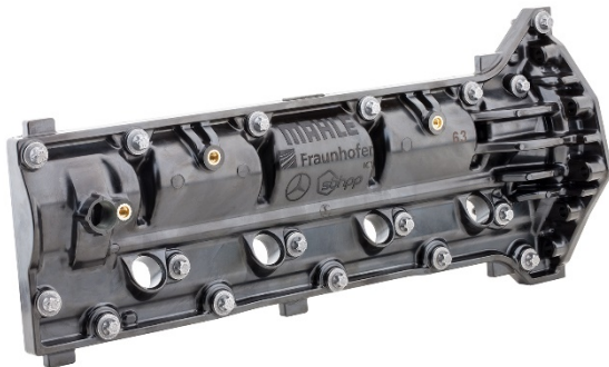
Picture 2: The fiber-reinforced thermoset polymer component lowers engine weight.
