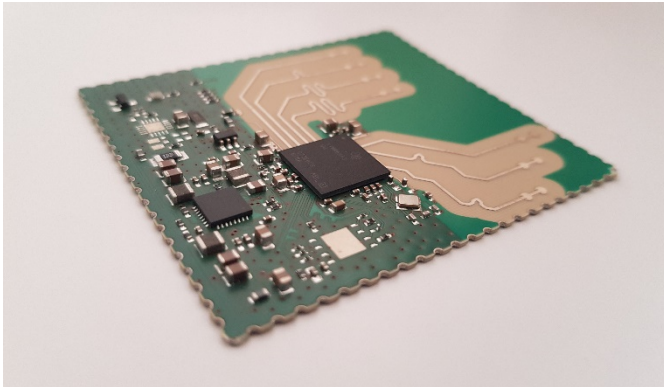
Fig. 2 Up to nine send/receive modules like these are integrated into the lamp structure. In this arrangement, they cover the entire room.
