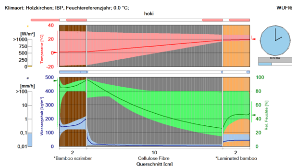
Fig. 2 The WUFI® software from Fraunhofer IBP shows a material's response to moisture over time by means of a film. The y axis indicates temperature and moisture content, while the x axis shows a cross-section of the component.
