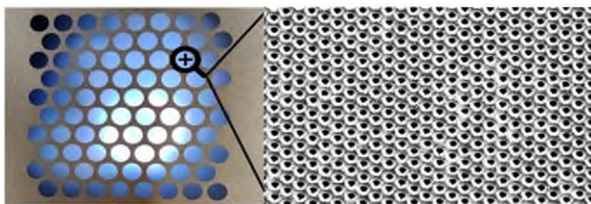
Figure 2: In the microplastic filter, the films with the microholes are fixed on a coarser grid so that they do not tear under the water pressure.
