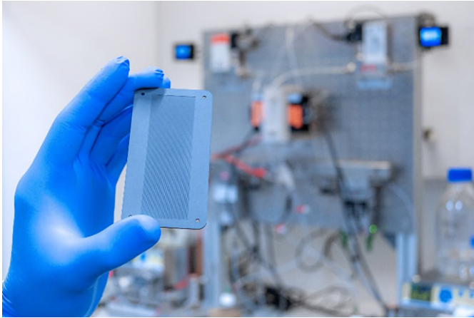
Fig. 2 A diamond-coated reaction plate with micro-channels as the key element for the continuously operated flow-through reactor which converts CO 2 into C 1 building blocks.
