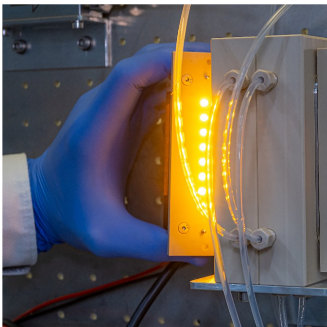
Fig. 1 Visible light as the energy source for the photocatalyzed conversion of CO 2 on diamond surfaces.
