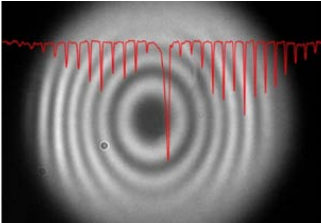
Picture 1 The invisible made visible: Using entangled photons and interference effects, infrared spectra of molecules (here: methane) can be recorded by cameras that can only detect visible light.
