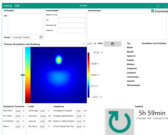
Abb. 2 FlareSimulator combines the factors of thermal convection and radiation and accurately calculates the heating of an object
