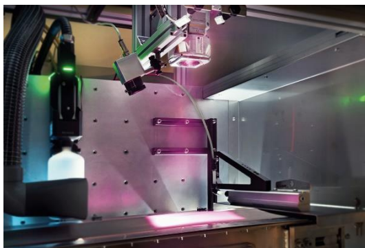
Fig. 1 Drying with diode lasers: Thanks to the special optics, the laser radiates a larger area on the copper foil coated with graphite paste. The interaction between the graphite particles and the light energy generates heat and the liquid evaporates.
